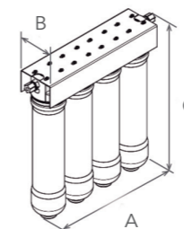
Water Stop 3/8''
